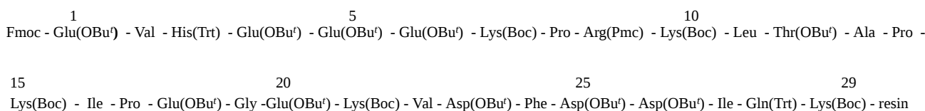
Scheme 2 Structure of the protected troponin-T 34–62 segment, synthesized on a p -benzyloxybenzyl alcohol polystyrene resin (Bu t = tert -butyl, Trt = trityl, Boc = tert -butoxycarbonyl, Pmc = 2,2,5,7,8-pentamethylchroman-6-sulfonyl)
