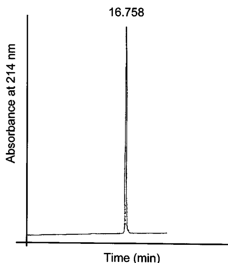
Fig. 3 HPLC profile of purified synthetic troponin-T 34–62 peptide fragment. Column: Nucleosil 100 C 18 (250 × 20 mm, 7 μm; Macherey-Nagel, Düren, Germany). Gradient: 5–90% B in 31 min; A: 0.05% TFA in H 2 O; B: 60% CH 3 CN, 0.08% TFA in H 2 O. Flow rate: 1mL/min. Detection: UV at λ = 214 nm
