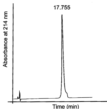
Fig. 8 HPLC profile of purified synthetic troponin-T 16–31 (1–16) fragment, isolated from TCA meat extracts. Column: Nucleosil 100 \text{C}_{18} (250 × 20 mm, 5 \mu\text{m} ; Macherey-Nagel, Düren, Germany). Gradient: 5–90%B in 36 min; A: 0.35% TFA in \text{H}_2\text{O} ; B: 60% \text{CH}_3\text{CN} , 0.29% TFA in \text{H}_2\text{O} . Flow rate: 1 mL/min. Detection: UV at \lambda = 214 nm
