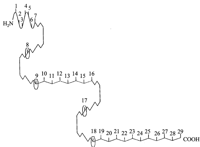
Fig. 2 Chou-Fasman secondary structure plot of the troponin-T fragment 34–62 of the following primary structure: ^{1(34)}EVHEE\text{-}EEKPR^{10}KLTAPKIP\text{-}EG^{20}EKVDFDDIQ^{29(62)}K . High antigenic index segments are marked by octagons; \sim : \alpha -helix, \subset : \beta -turn, \wedge : random coil structure
