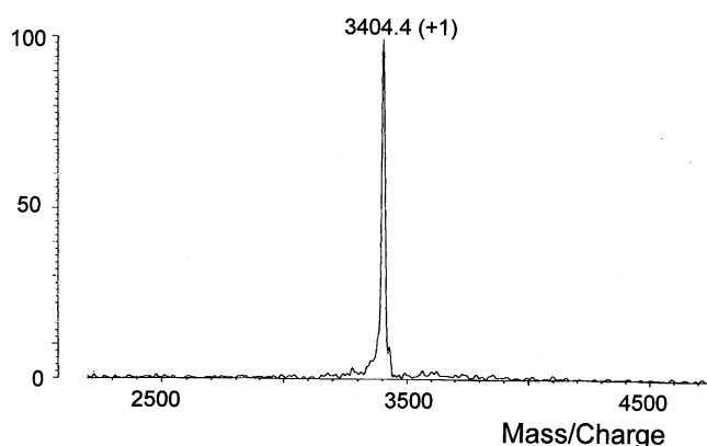
Fig. 4 MALDI spectrum of purified synthetic troponin-T 34–62 peptide fragment. Wavelength: 337 nm. Matrix: \alpha -cyano-4-hydroxycinnamic acid
