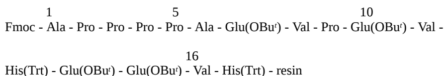
Scheme 3 Structure of the protected troponin-T 16–31 (1–16) segment, isolated from meat TCA extracts and synthesized on a p -benzyloxybenzyl alcohol polystyrene resin ( \text{Bu}^t = tert -butyl, Trt = trityl).
