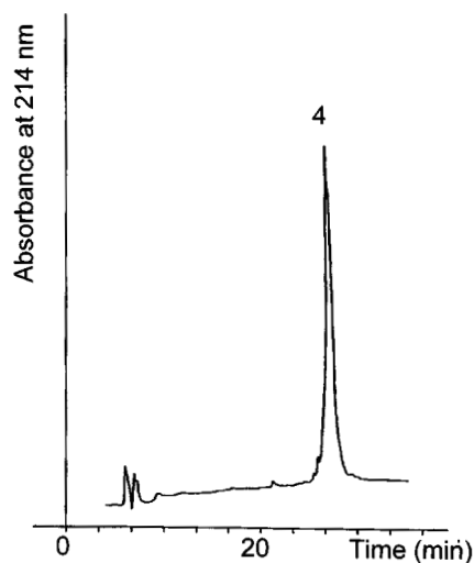
Fig. 11 HPLC profile of pooled fraction 4 (Figure 6) of TCA meat extracts. Column: LiChrospher RP-18 (250 × 4 mm, 5 μm; Merck). Gradient: 5–60% B in 60 min; A: 0.1% TFA in H 2 O, B: 80% CH 3 CN, 0.1% TFA in H 2 O. Flow rate: 1 mL/min. Injection volume: 100 μL. Detection: UV at λ = 214 nm
