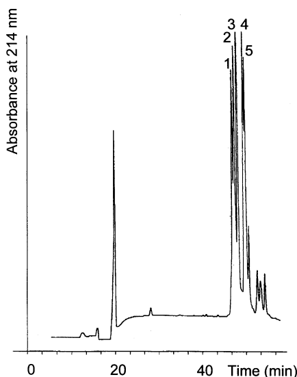
Fig. 15 HPLC profile of HCl-soluble extract of a beef sample after storage for 3 days. 250 \mu\text{g} / 250 \mu\text{L} (Fraction 3, see Figure 14) were injected into the Rhodyne valve. Column: Nucleosil 100 RP-18 (250 \times 10 mm; 7 \mu\text{m} ; Macherey-Nagel, Düren, Germany). Gradient: 15 to 100% B in 60 min; A: 0.1% TFA in \text{H}_2\text{O} , B: 80% \text{CH}_3\text{CN} , 0.1% TFA in \text{H}_2\text{O} . Flow rate: 1.0 mL/min. Detection: UV at \lambda = 214 \text{ nm} (Concerning numbering of the peaks, see text)
