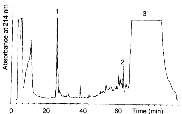
Fig. 14 HPLC profile of HCl-soluble extract of a beef sample after storage for 3 days. 150 \mu\text{L} of the extract were diluted injected into the Rhodyne valve. Column: LiChrospher RP-18 (250 \times 4 mm, 5 \mu\text{m} ; Merck). Gradient: 0 to 70% B in 60 min; A: 0.1% TFA in \text{H}_2\text{O} , B: 80% \text{CH}_3\text{CN} , 0.1% TFA in \text{H}_2\text{O} . Flow rate: 1.0 mL/min. Detection: UV at \lambda = 214 \text{ nm}
